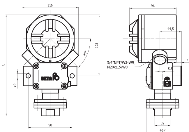
“W” - Series: Pressure & Vacuum “P...V/M”
