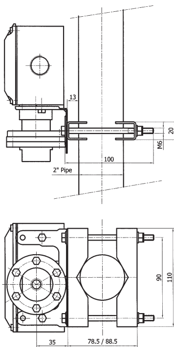
"C."- Series Enclosure on 2" Pipe
