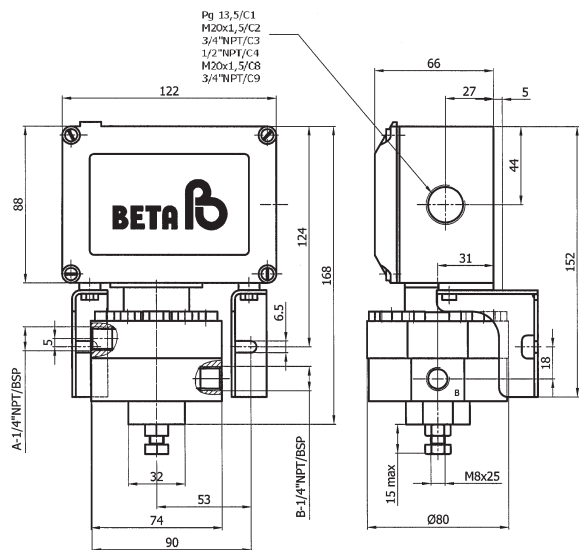
“C” - Series: Bi-directional Differential “D...D”
