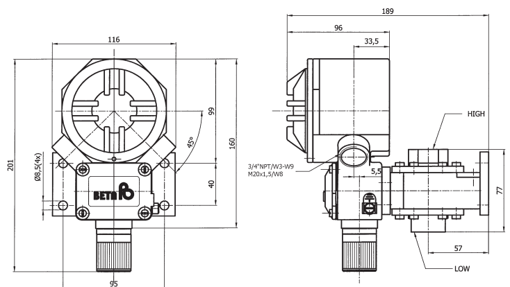
“W” - Series: Differential “D...M”
