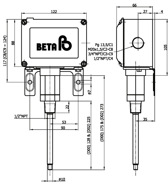
“C” - Series: Temperature “T..H - D”
