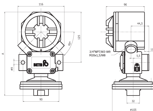
“W” - Series: Pressure & Vacuum “P...V/L”
