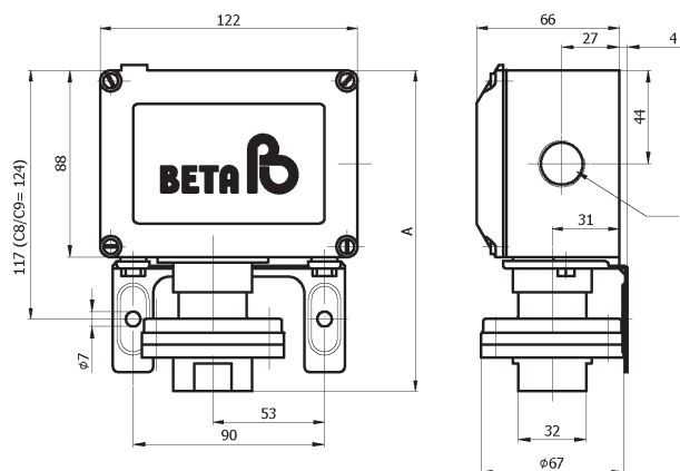
“C” - Series: Pressure & Vacuum “P...V/M”
