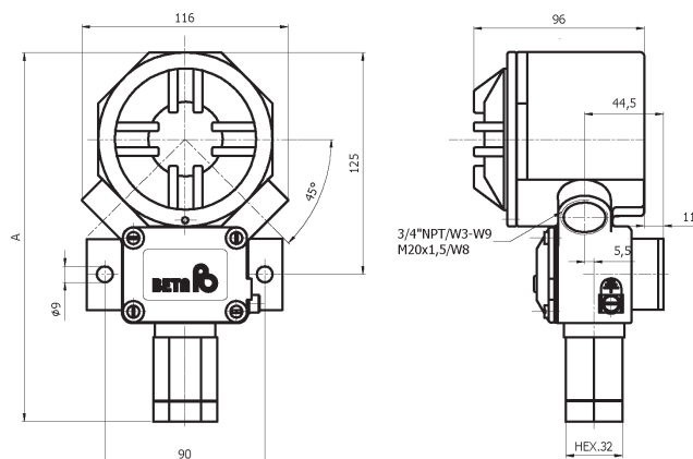
“W” - Series: Pressure & Vacuum “P...V/H”
